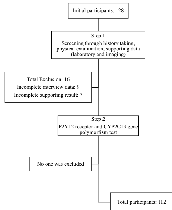
Fig. 1 Subject screening
